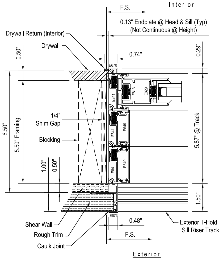
(E673) 1.00" Exterior Trim w/ 1.50" Wide (E643ADA) Exterior T-Hold Sill Riser Profile Multi-Slide Stacking Door Jamb Application
