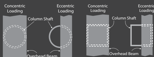
Tapered & Non-tapered Round FRP Column
