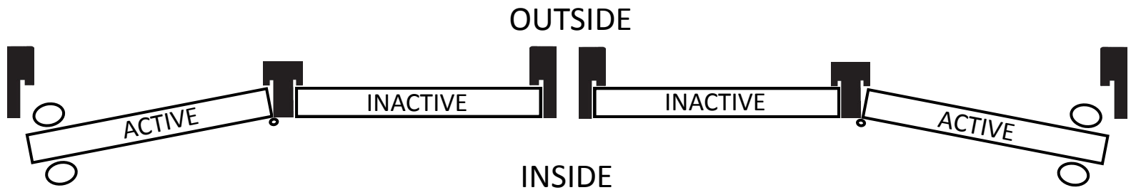
LEFT HAND CENTER HINGED INSWING
