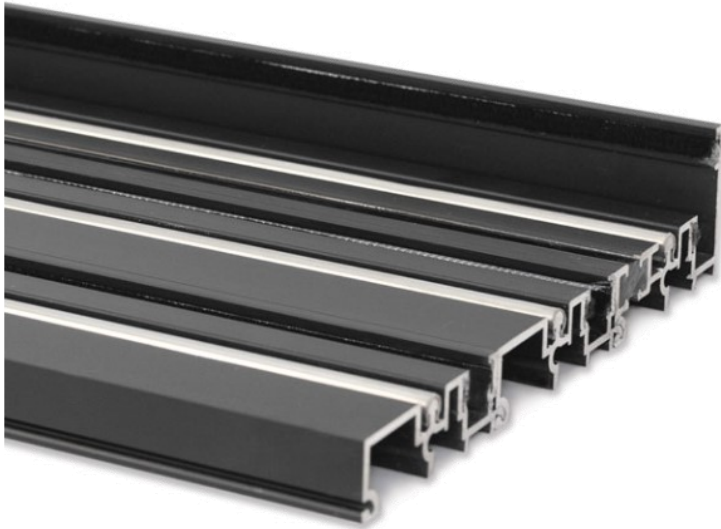
WATER BARRIER SILL
